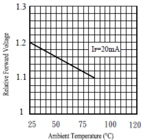
Fig.5 Forward Voltage vs. Ambient Temperature (°C)
