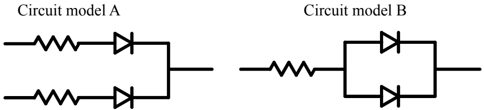
(A)Recommended circuit.
