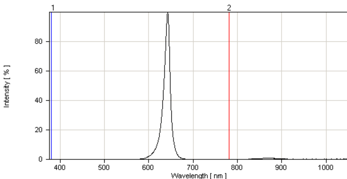
Fig.1 Red Relative Intensity vs. Wavelength
