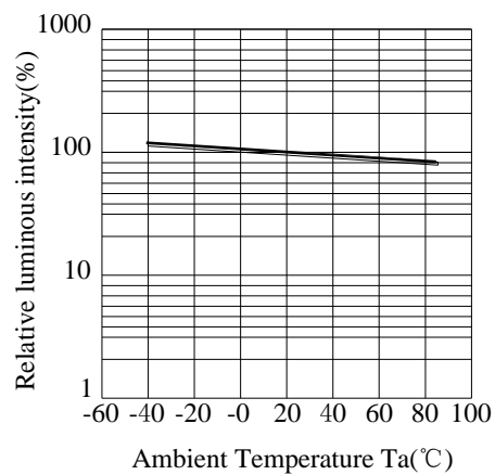
Fig.3 Luminous Intensity vs. Ambient Temperature
