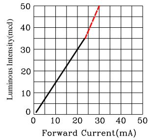
Fig.3 Luminous Intensity vs. Forward Current
