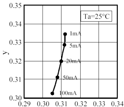
■ Forward Current vs. Chromaticity Coordinate
