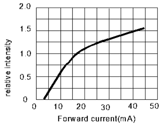
Relative light intensity vs current
