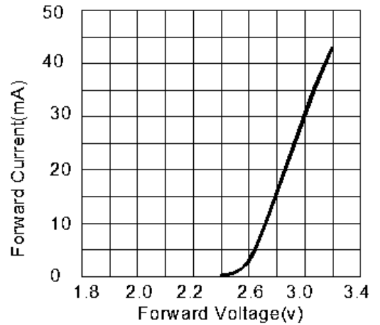
Voltage current relationship
