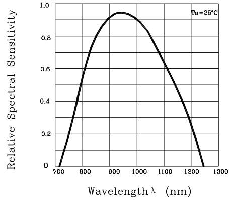
Fig. 2 Spectral Sensitivity
