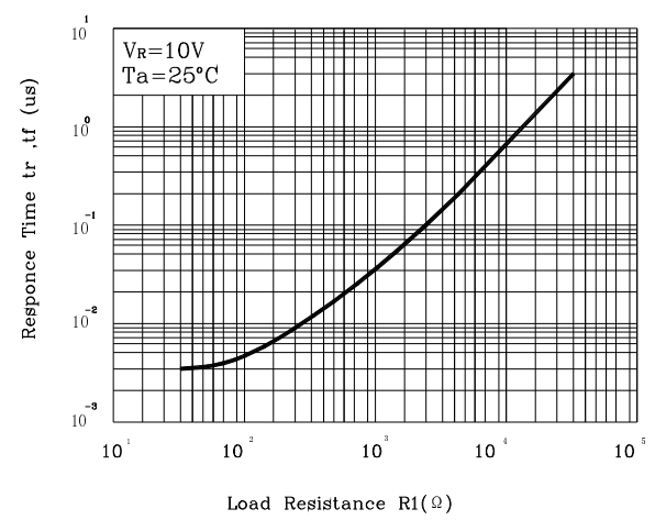
Fig. 6 Responce Time vs Load Resistance
