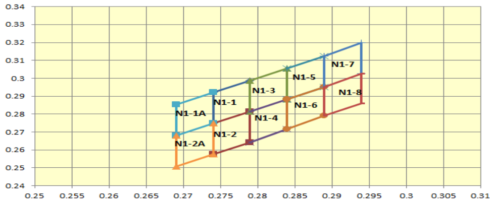
Color Rank (CIE chromaticity X , Y) @ 5mA
