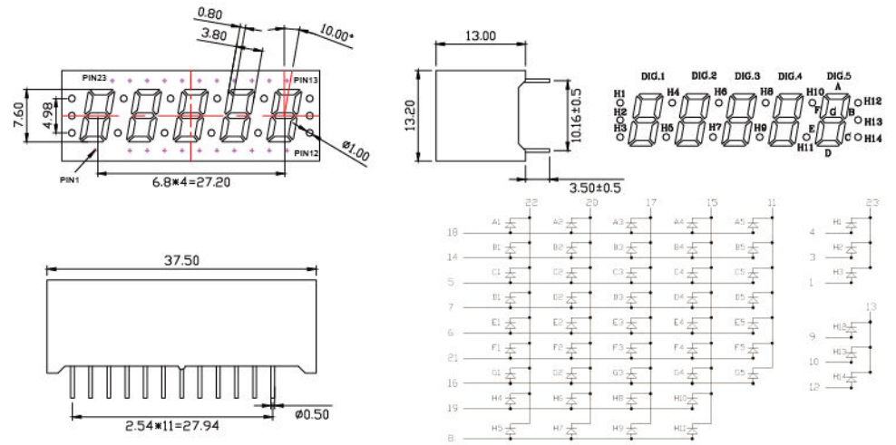
DSC53LR200G Outline Dimensions 0.3 inch
