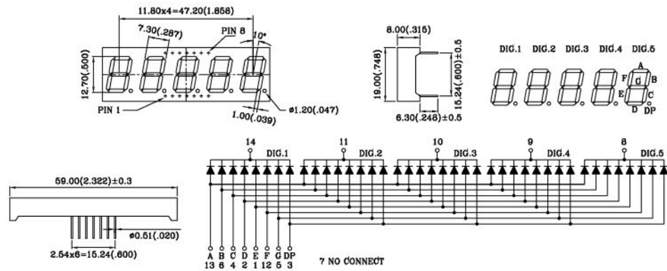
505 Outline Dimensions 0.5 inch
