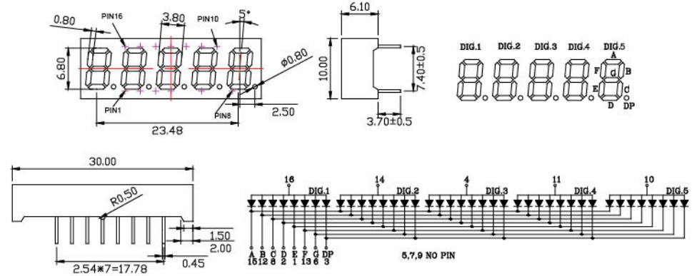
DSA52LR201G Outline Dimensions 0.27 inch
