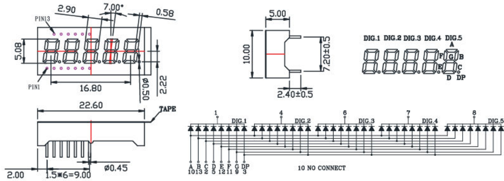
DSC52LR199G Outline Dimensions 0.2 inch
