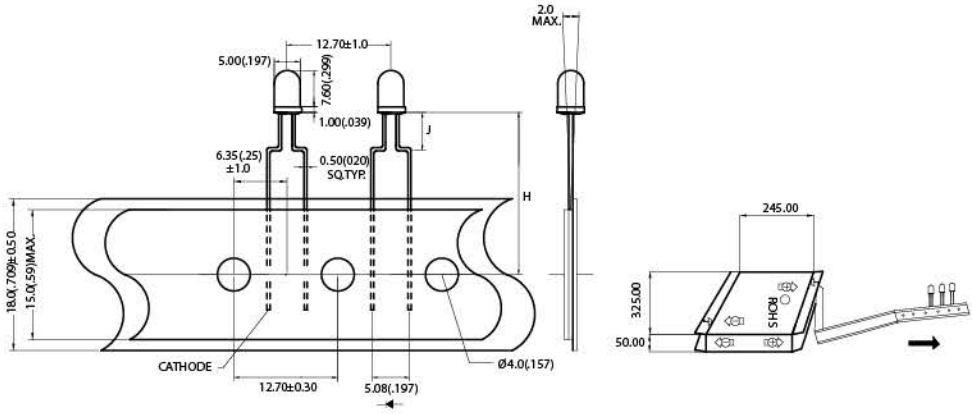
Outline Dimensions 5 mm
