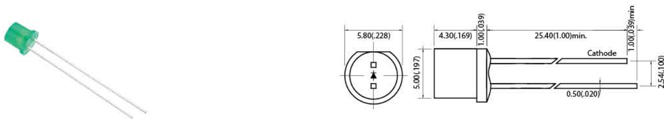
Outline Dimensions 5 mm
