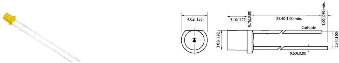
Outline Dimensions 3 mm
