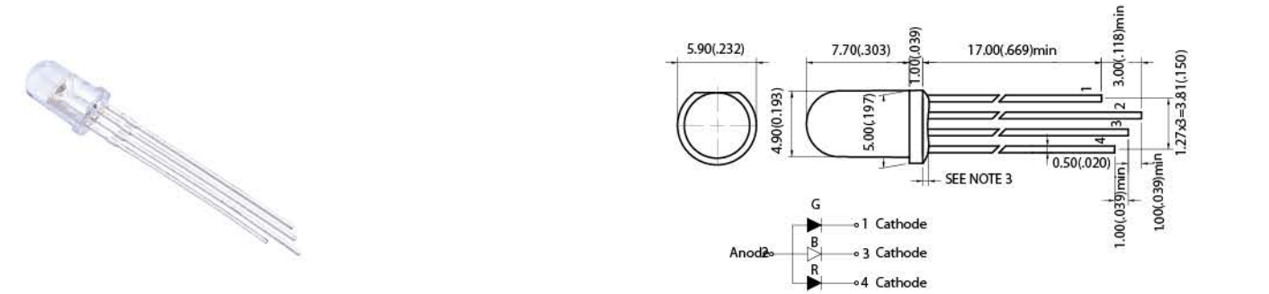
Outline Dimensions 5 mm
