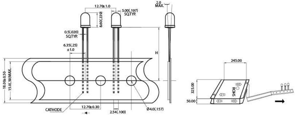
Outline Dimensions 5 mm
